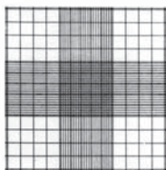
Neubauer Improved Counting Chamber
